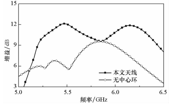
图 8 本文天线与无中心环馈电阵列的仿真增益变化 Fig. 8 Simulated gains of the proposed antenna and the patch array without mental square ring
