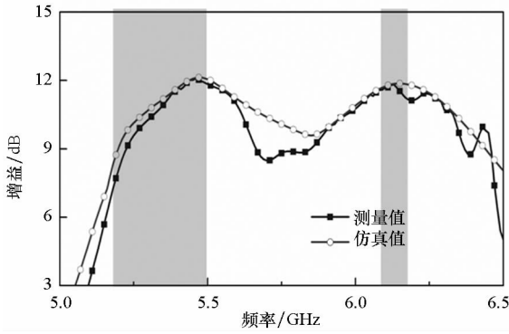
图 6 微带贴片阵列仿真及测量增益随频率的变化 Fig. 6 Simulated and measured gains of the patch array
