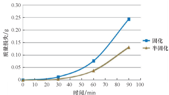
(a) 两种不同涂层的平均质量损失与时间的关系 (a) Relationship between the average mass loss and time for two different coatings
