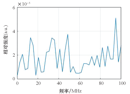
图 4 400 ns 单脉冲发射频域信号 Fig. 4 Signal of 400 ns single pulse emission in frequency domain
