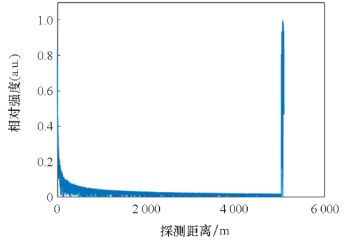
图 3 400 ns 单脉冲发射时域回波信号 Fig. 3 Echo signal of 400 ns single pulse emission in time domain
